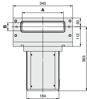
Valve seat side (XGT222, 223, and 224 common)
