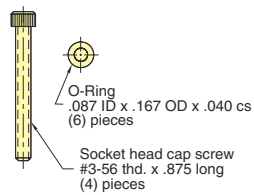
Mounting hardware
