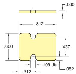
Cover plate
