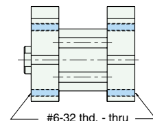
Thread Mount AF-Txx-17-x
