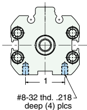
Bottom Mount AF-Bxx-17-x
