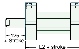
Spring Extend AF-xRR-12-x
