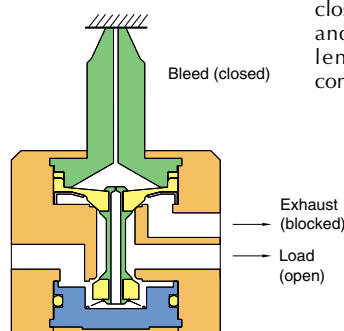
Valve Open
