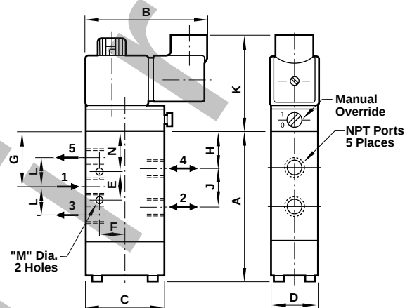
Fig. 5 – 1/2" valve solenoid-air return
