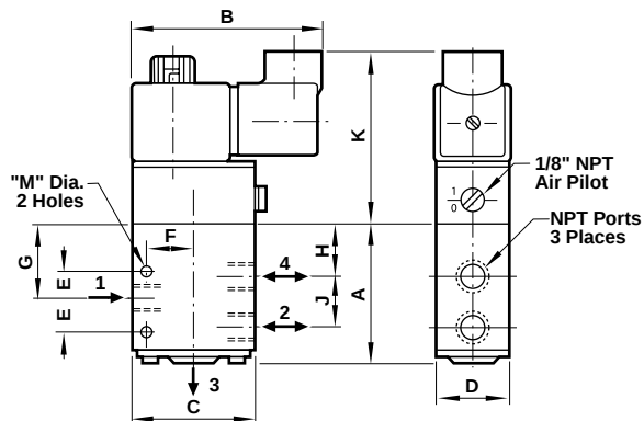
Fig. 2 – 1/8" valve solenoid-air return
