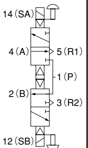
Normally closed (NC), Normally open (NO)
