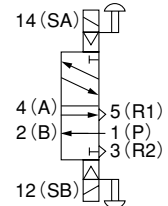
HJA10A6 De-energized condition after energizing solenoid 12(SB)
