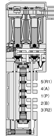
HJA10A6 De-energized condition after energizing solenoid 12(SB)
