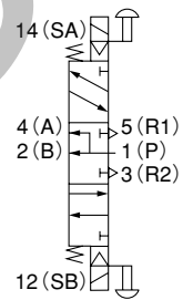
PAB connection
