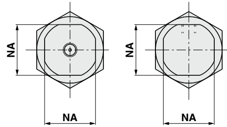
Head cover axial port Boss-cut/Basic
