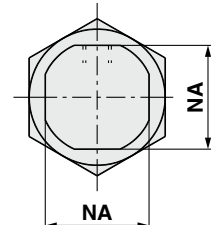
Boss-cut/Basic
