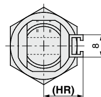
Rail mounting (A)
