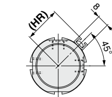
Rail mounting (A)
