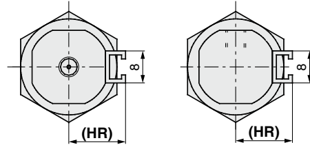
Head cover axial port Boss-cut/Basic
