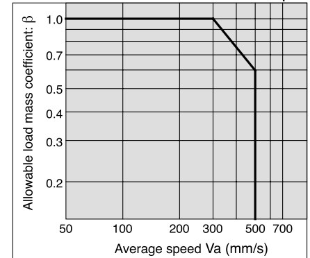
Graph (1) Allowable Load Mass Coefficient: \beta
