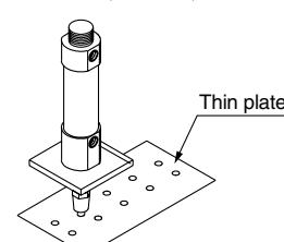
Punching
