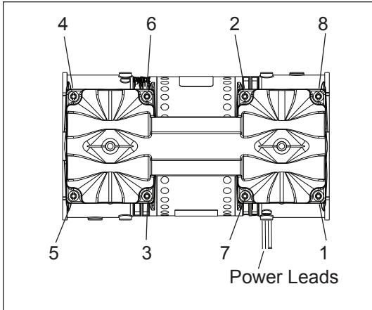
Numbers indicate tightening sequence Head Assembly
