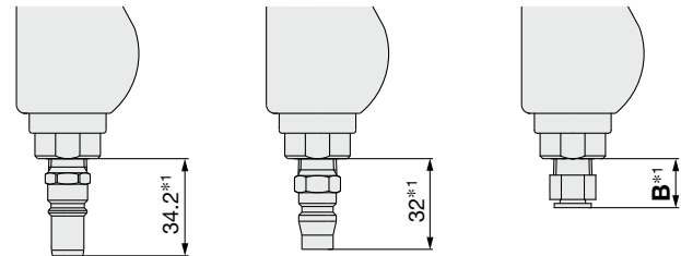
S coupler plug mounting (KK4P-02MS)
