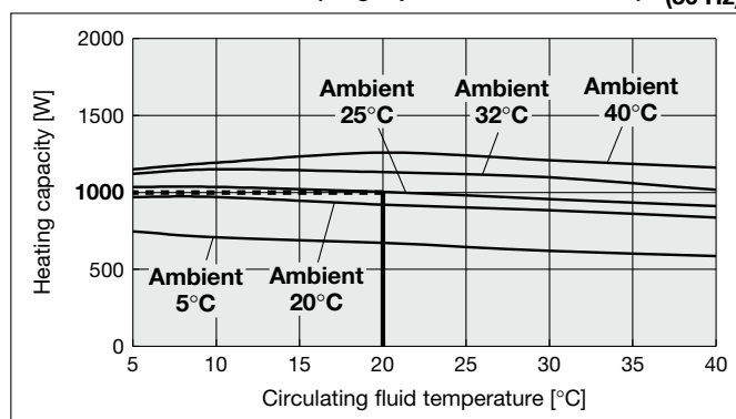
HRSF050/060-A-20 (Single-phase 200 to 230 VAC)
