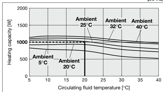
HRSF060-W-20 (Single-phase 200 to 230 VAC)
