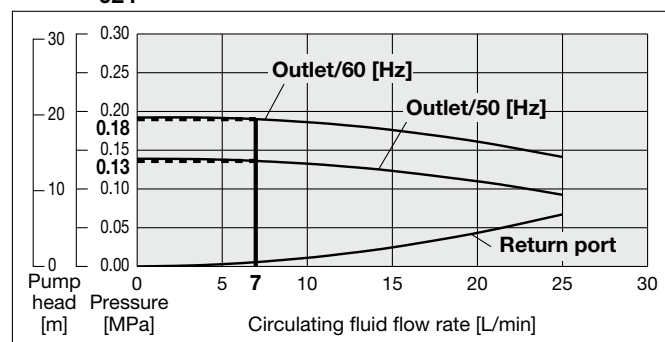
HRSF 012 018 -A W -20 (Single-phase 200 to 230 VAC)
