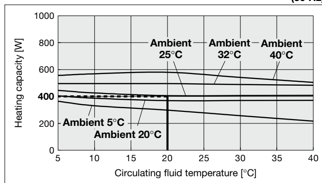
HRSF030-W-20 (Single-phase 200 to 230 VAC)
