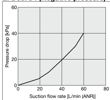
ZFD53: ø4 (Negative pressure)
