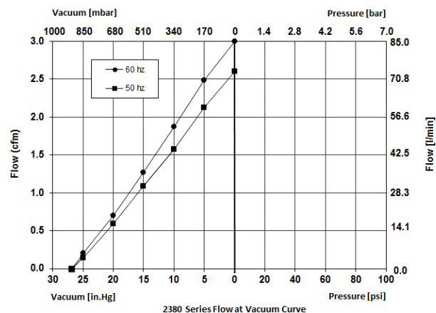
2380 Series Flow at Vacuum Curve
